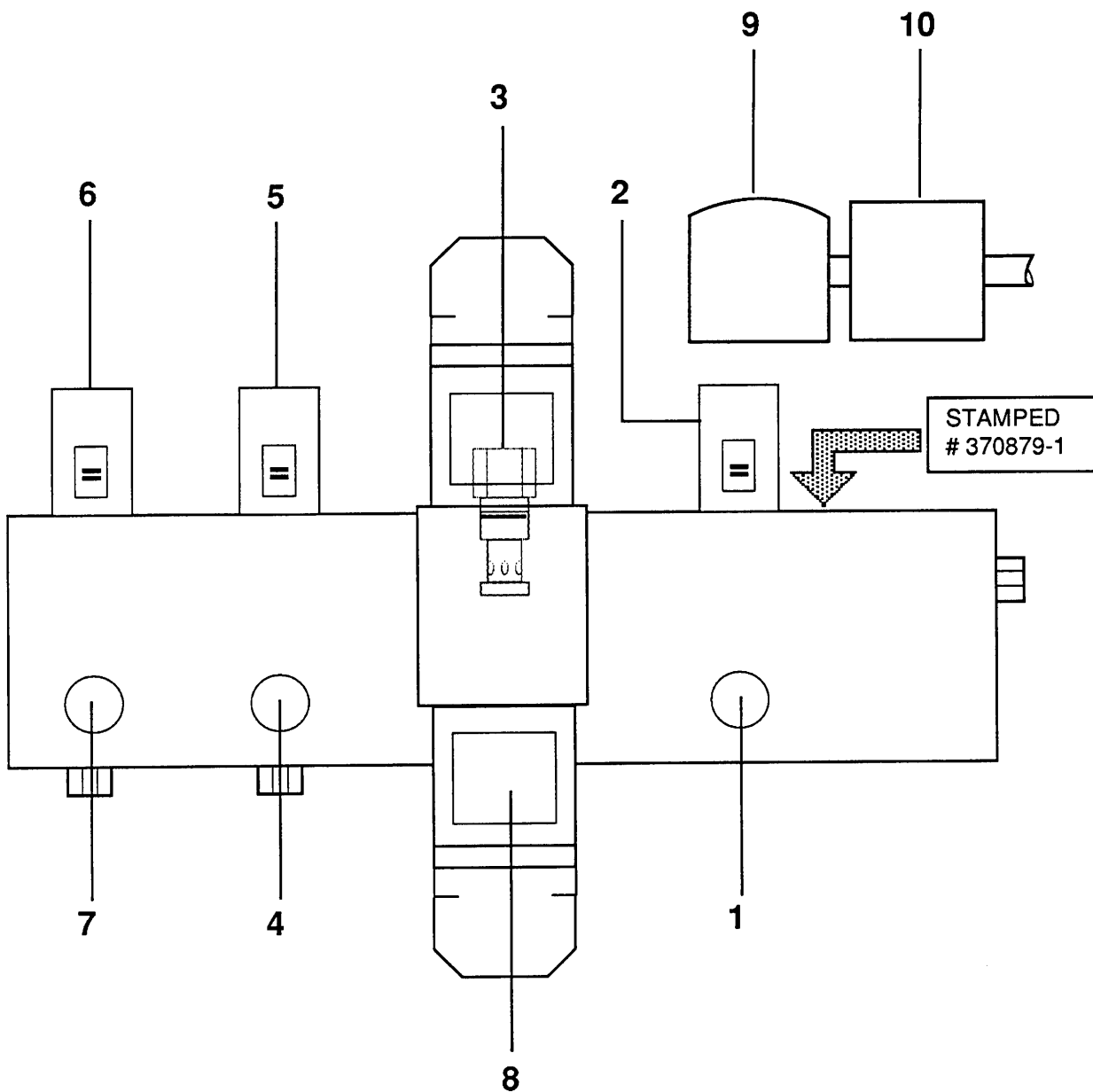
TOP VIEW
